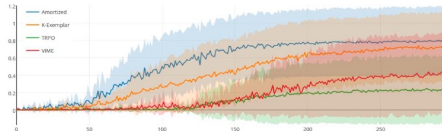
Figure 9: DoomMyWayHome+
